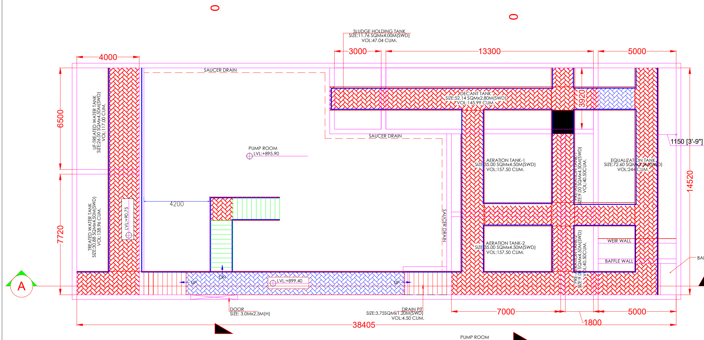
410 KLD STP PLAN AT PLATFORM LEVEL
